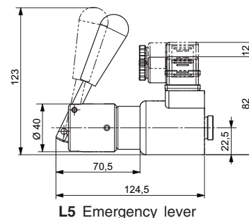
L5 Emergency lever
