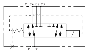
WITHOUT DRAINAGE - Y PLUGED
